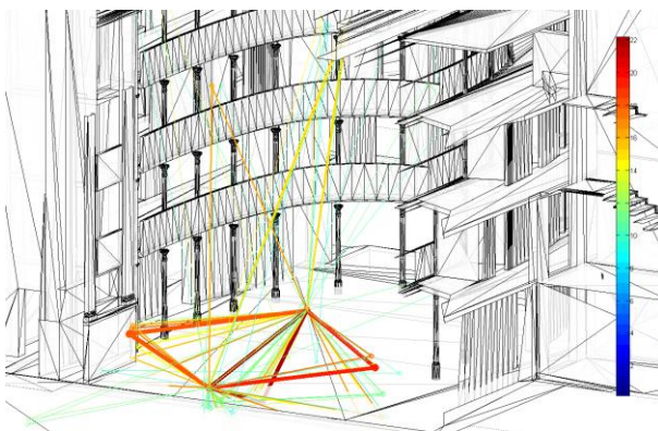
Figure 25: Trajectory analysis up to triple reflections based on MIMO IR measurement
