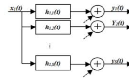
Figure 3: Scheme of the signal processor for a loudspeaker array
