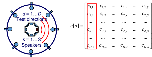
Figure 4: Loudspeaker array characterization
