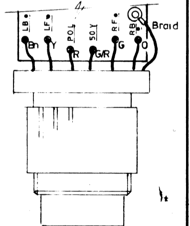
Rear elev. viewed from ("rear of mic")
